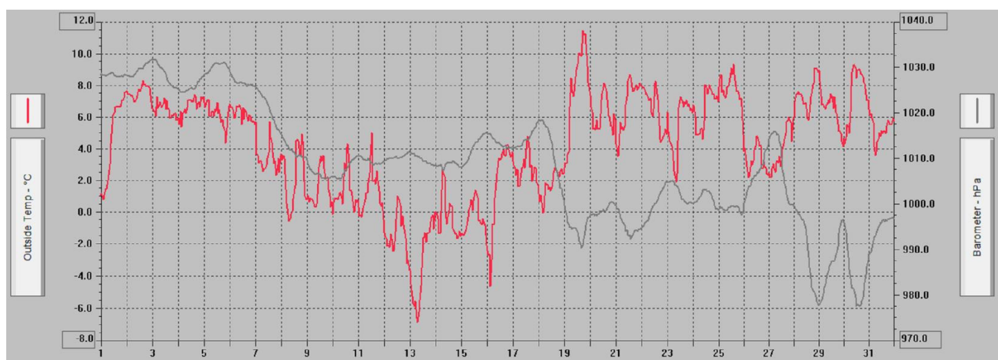
Figure 3: December temperature (Red) and barometer trace (Grey)
